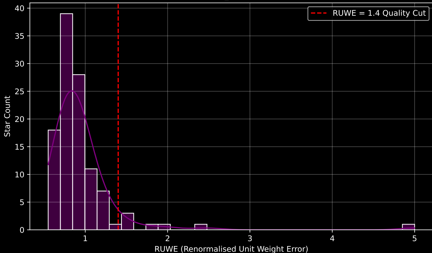
GAPOGEE DR17 Field [279-34-O_TESS] RUWE Distribution (n= 111)
